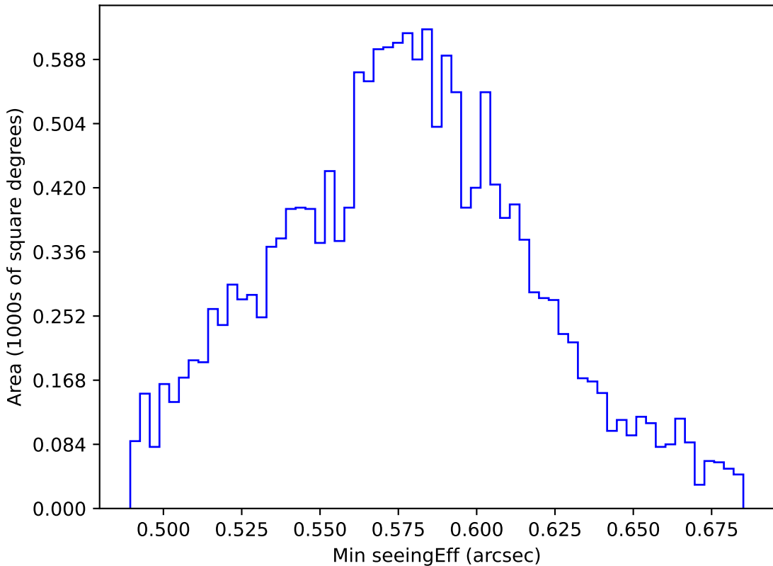
too_elab_r8_d3_griz_v3.4_10yrs WFD all bands: Min seeingEff
