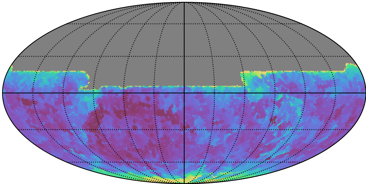
too_elab_r8_d3_griz_v3.4_10yrs All sky y band: Min seeingEff
