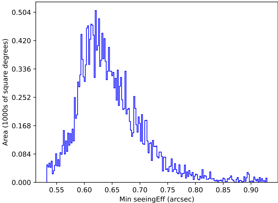
too_elab_r8_d3_griz_v3.4_10yrs All sky y band: Min seeingEff
