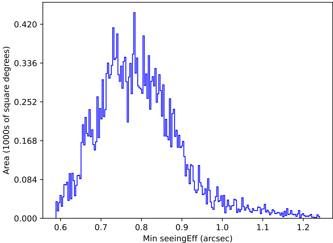
too_elab_r8_d3_griz_v3.4_10yrs All sky u band: Min seeingEff
