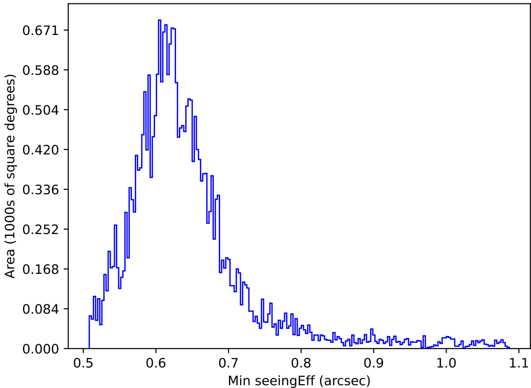
too_elab_r8_d3_griz_v3.4_10yrs All sky r band: Min seeingEff
