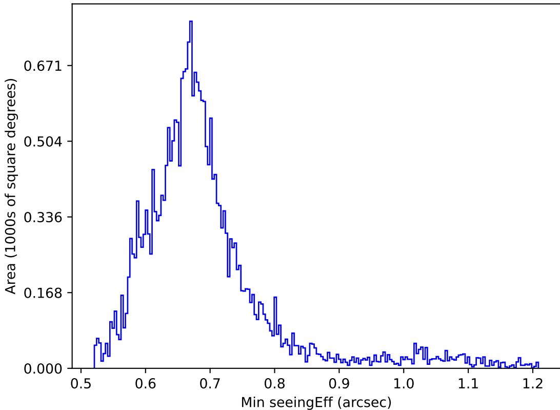
too_elab_r8_d3_griz_v3.4_10yrs All sky g band: Min seeingEff
