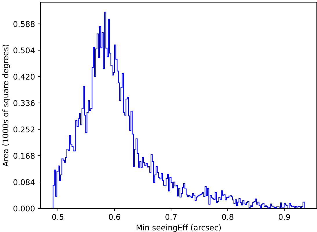
too_elab_r8_d3_griz_v3.4_10yrs All sky all bands: Min seeingEff
