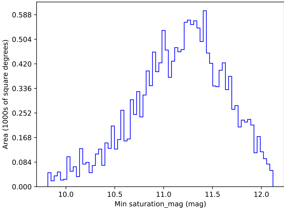
too_elab_r8_d3_griz_v3.4_10yrs WFD y band: Min saturation_mag
