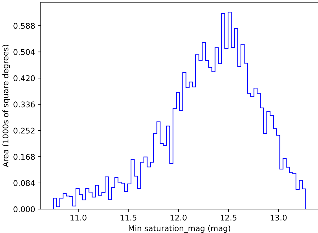
too_elab_r8_d3_griz_v3.4_10yrs WFD i band: Min saturation_mag
