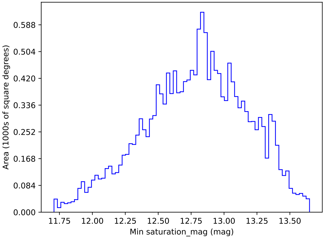
too_elab_r8_d3_griz_v3.4_10yrs WFD g band: Min saturation_mag
