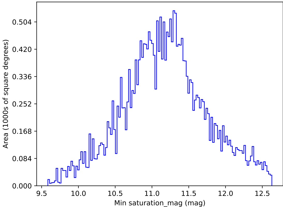
too_elab_r8_d3_griz_v3.4_10yrs All sky all bands: Min saturation_mag
