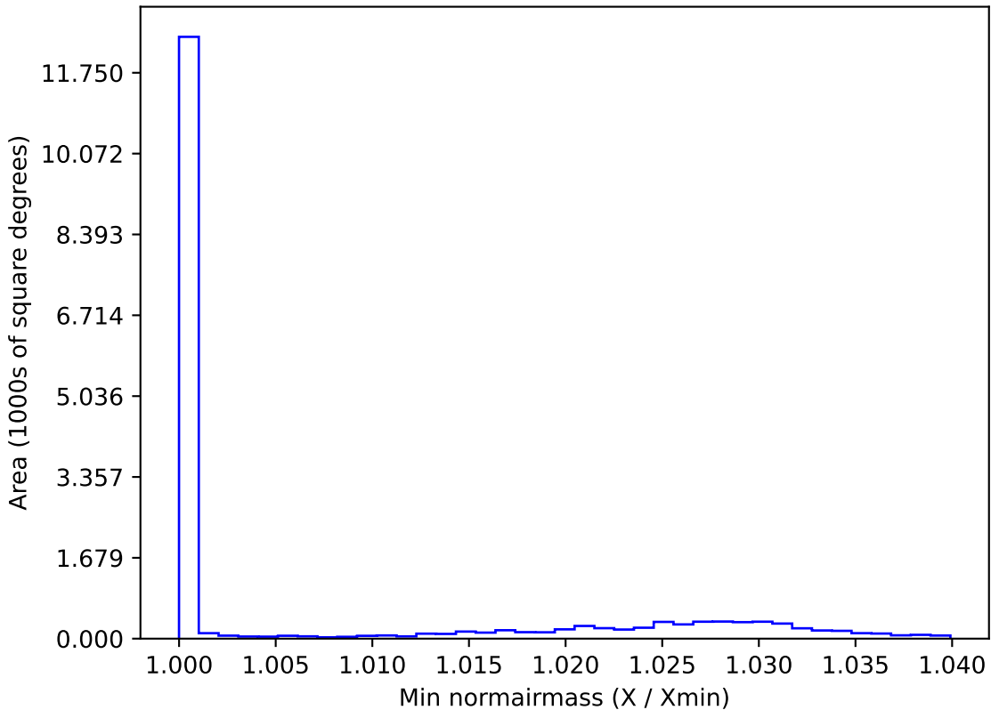
too_elab_r8_d3_griz_v3.4_10yrs WFD y band: Min normairmass
