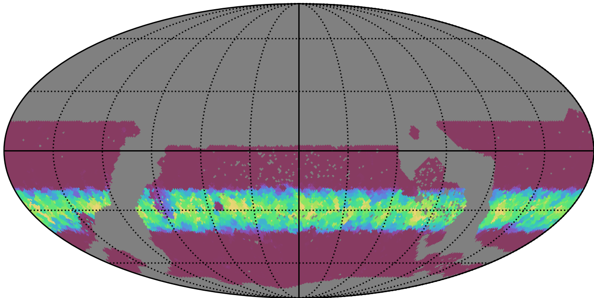
too_elab_r8_d3_griz_v3.4_10yrs WFD g band: Min normairmass
