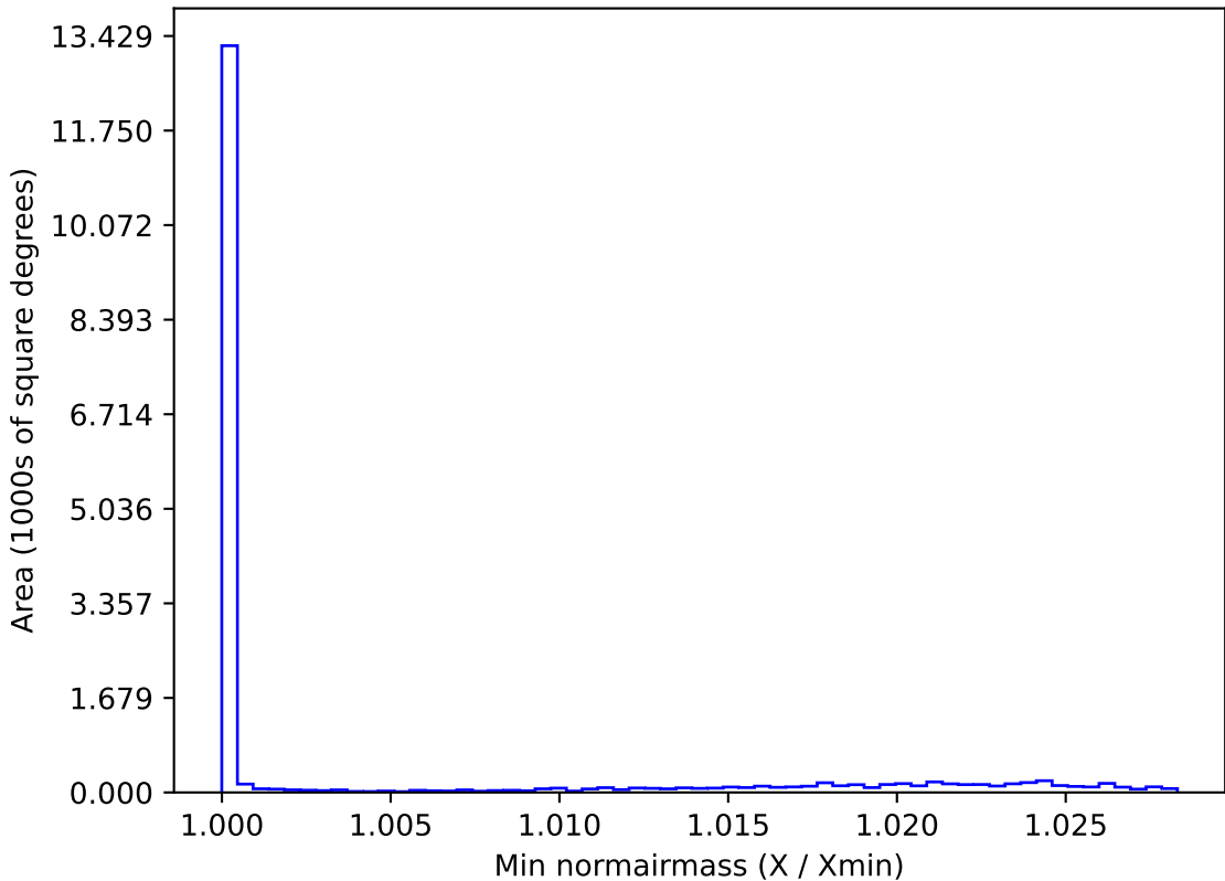
too_elab_r8_d3_griz_v3.4_10yrs WFD all bands: Min normairmass
