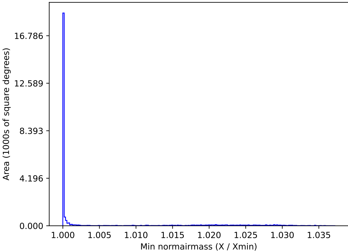
too_elab_r8_d3_griz_v3.4_10yrs All sky r band: Min normairmass
