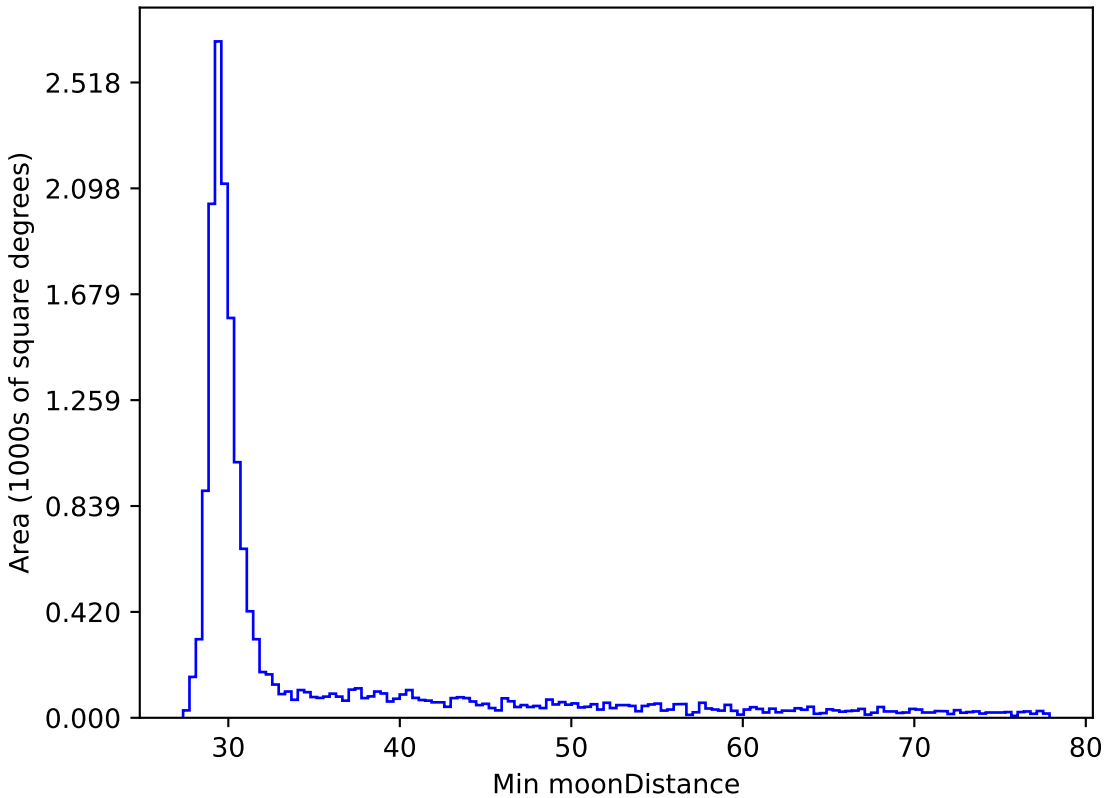
too_elab_r8_d3_griz_v3.4_10yrs WFD z band: Min moonDistance
