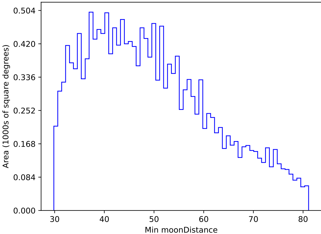
too_elab_r8_d3_griz_v3.4_10yrs WFD u band: Min moonDistance
