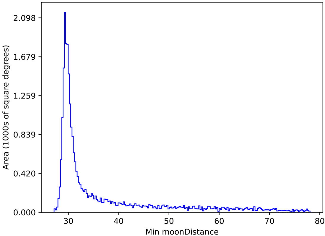
too_elab_r8_d3_griz_v3.4_10yrs All sky z band: Min moonDistance
