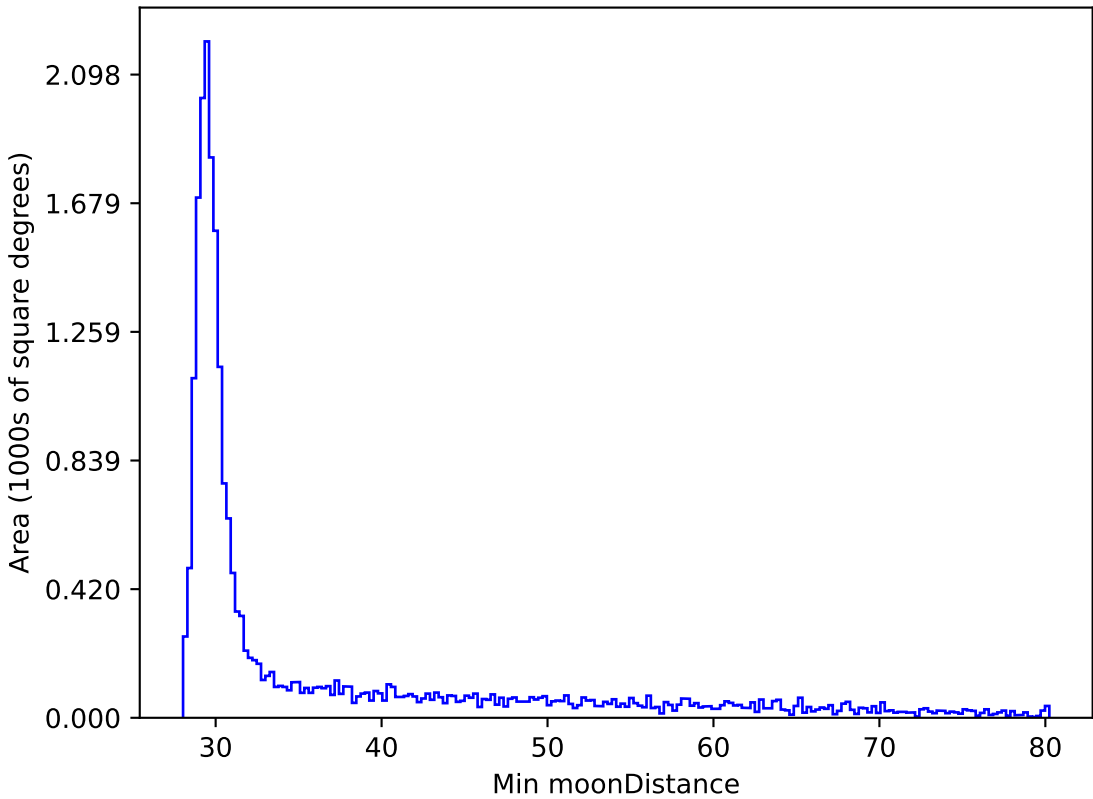
too_elab_r8_d3_griz_v3.4_10yrs All sky y band: Min moonDistance
