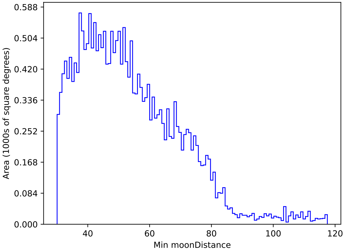
too_elab_r8_d3_griz_v3.4_10yrs All sky u band: Min moonDistance
