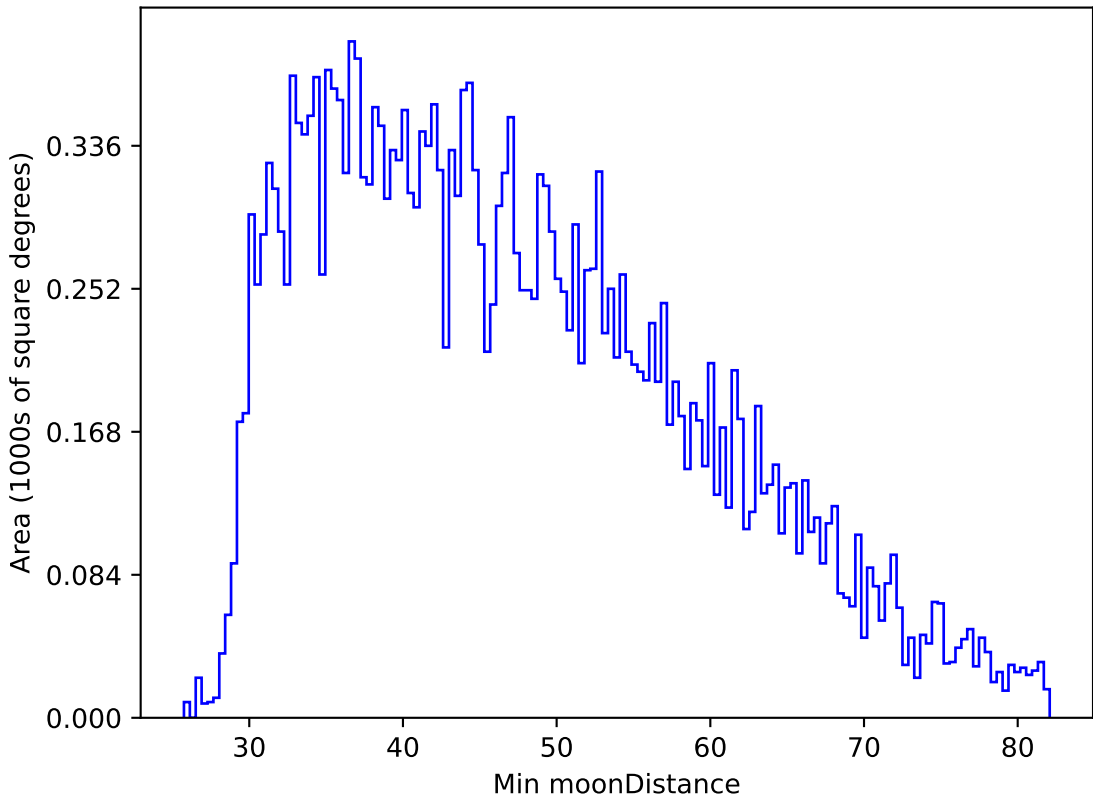
too_elab_r8_d3_griz_v3.4_10yrs All sky g band: Min moonDistance
