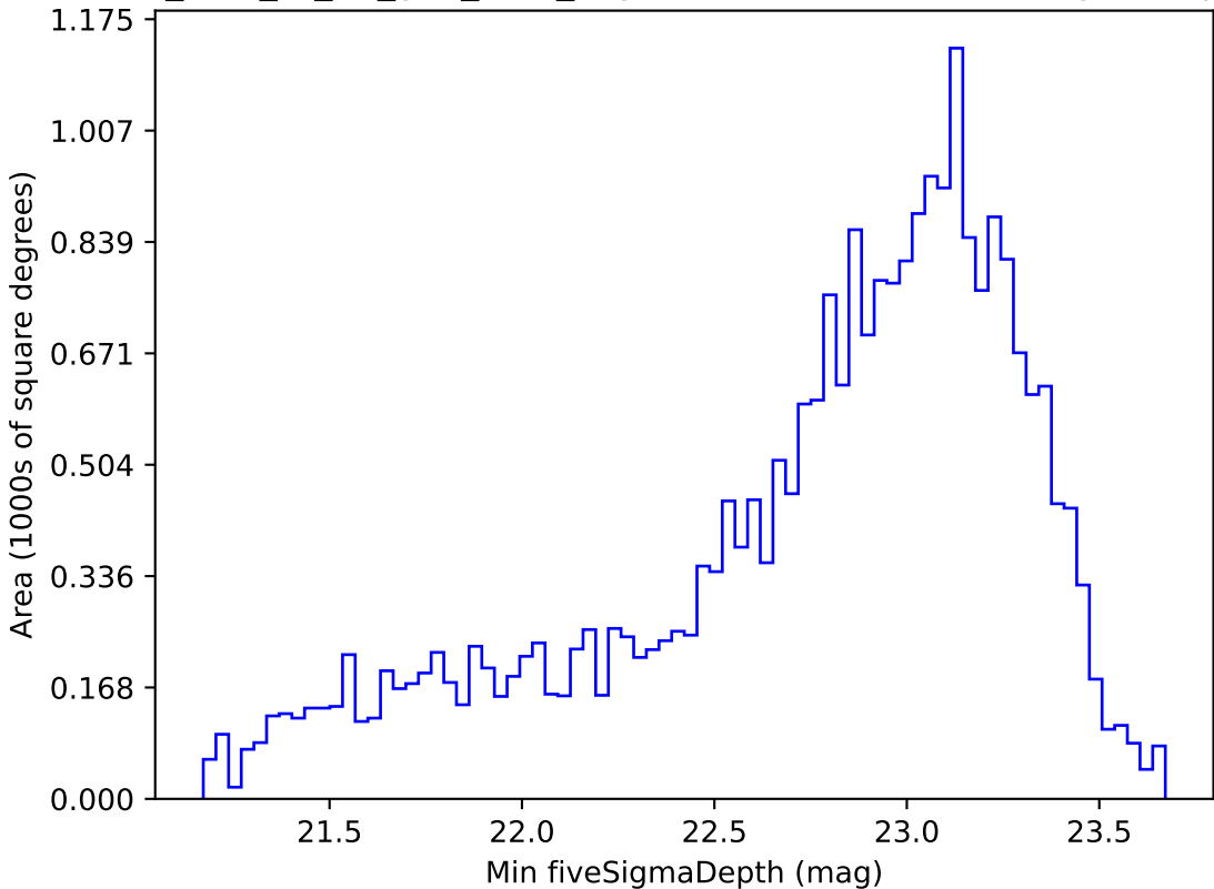
too_elab_r8_d3_griz_v3.4_10yrs Yr 1 i band: Min fiveSigmaDepth
