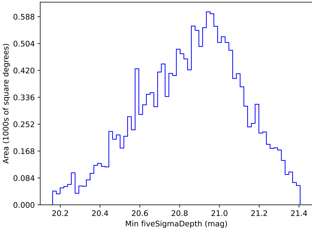
too_elab_r8_d3_griz_v3.4_10yrs WFD y band: Min fiveSigmaDepth
