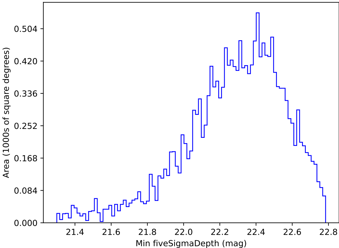
too_elab_r8_d3_griz_v3.4_10yrs WFD u band: Min fiveSigmaDepth
