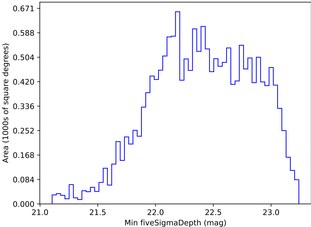
too_elab_r8_d3_griz_v3.4_10yrs WFD r band: Min fiveSigmaDepth
