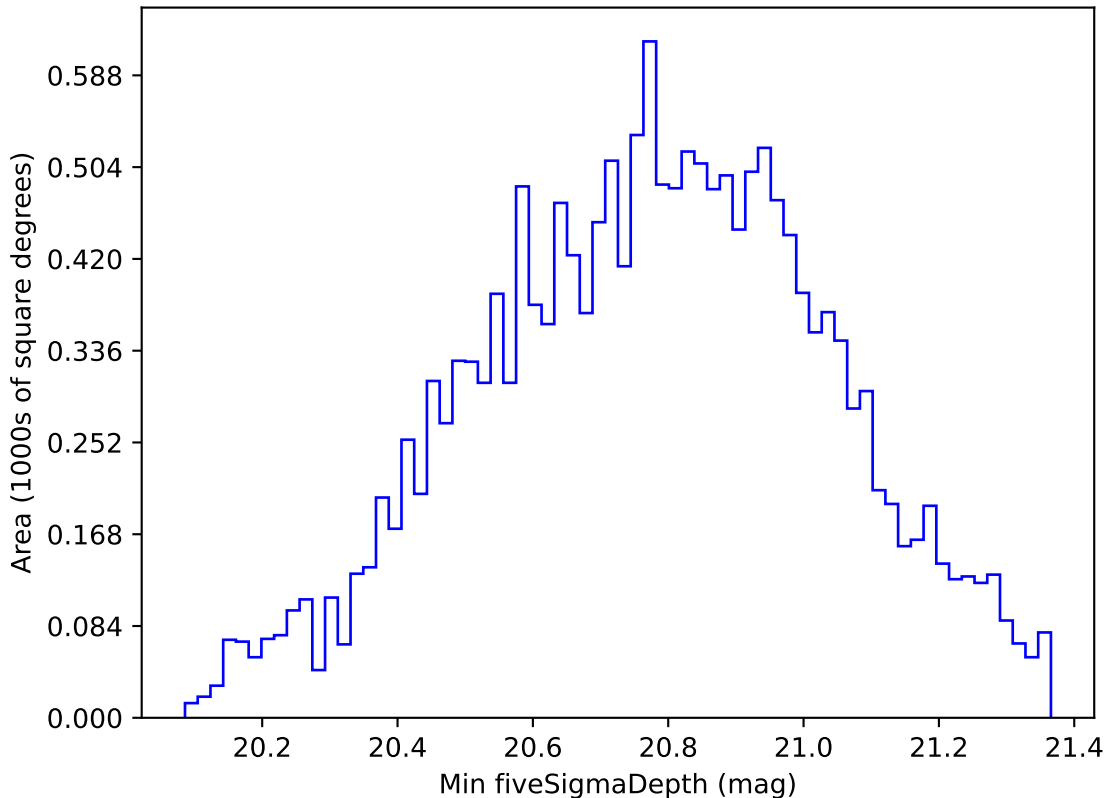
too_elab_r8_d3_griz_v3.4_10yrs WFD all bands: Min fiveSigmaDepth
