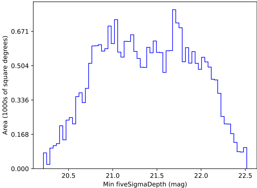
too_elab_r8_d3_griz_v3.4_10yrs All sky z band: Min fiveSigmaDepth
