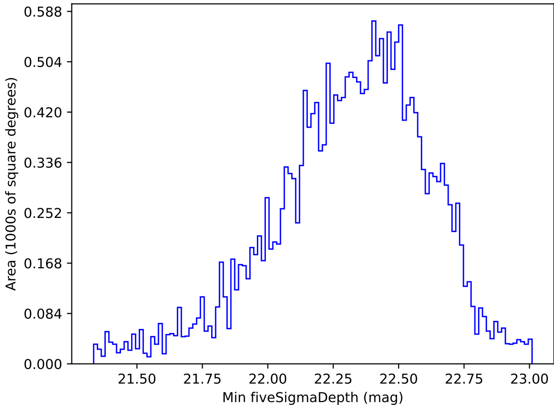
too_elab_r8_d3_griz_v3.4_10yrs All sky u band: Min fiveSigmaDepth
