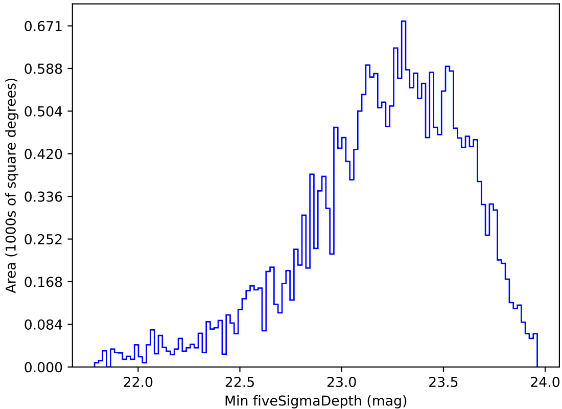
too_elab_r8_d3_griz_v3.4_10yrs All sky g band: Min fiveSigmaDepth
