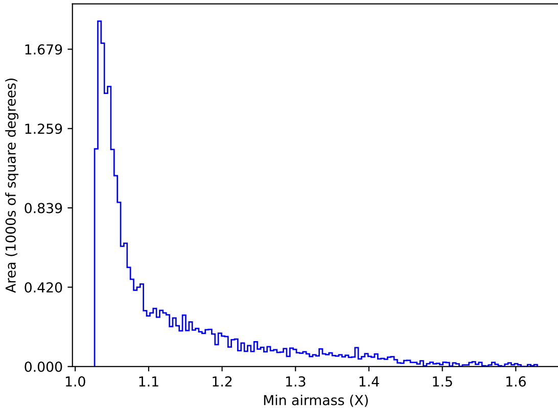
too_elab_r8_d3_griz_v3.4_10yrs Yr 1 y band: Min airmass
