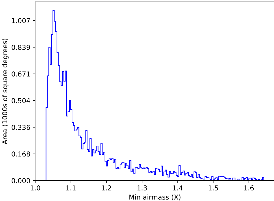
too_elab_r8_d3_griz_v3.4_10yrs Yr 1 u band: Min airmass
