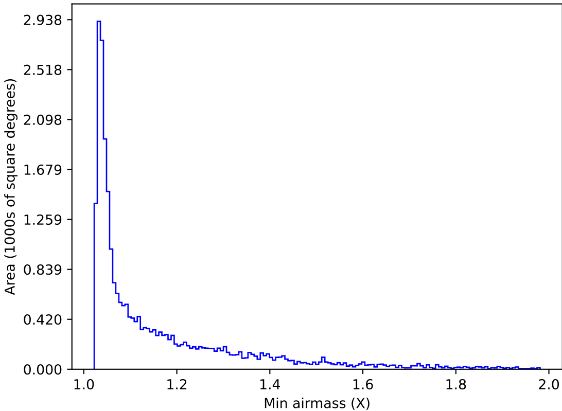
too_elab_r8_d3_griz_v3.4_10yrs Yr 1 r band: Min airmass
