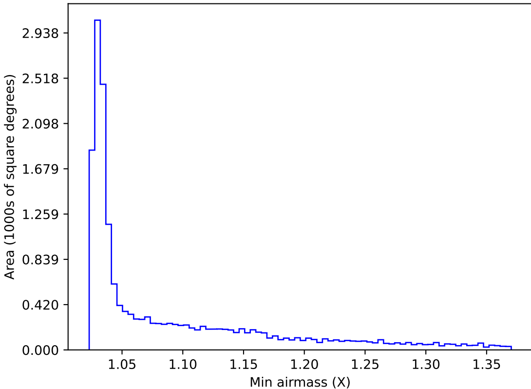
too_elab_r8_d3_griz_v3.4_10yrs WFD y band: Min airmass
