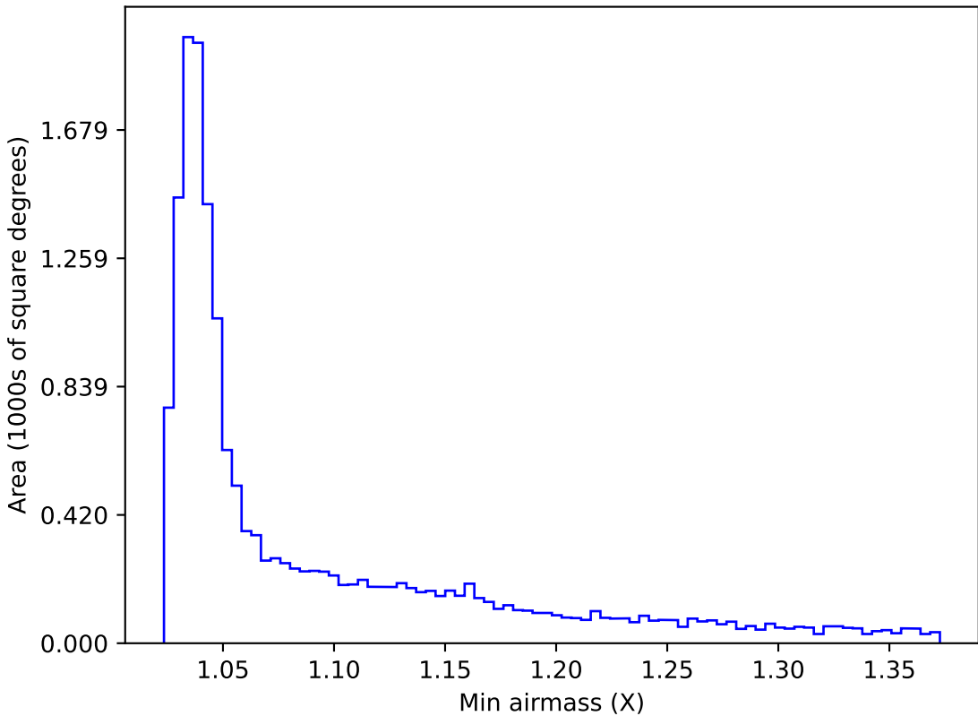
too_elab_r8_d3_griz_v3.4_10yrs WFD u band: Min airmass
