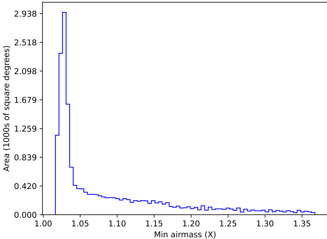
too_elab_r8_d3_griz_v3.4_10yrs WFD r band: Min airmass
