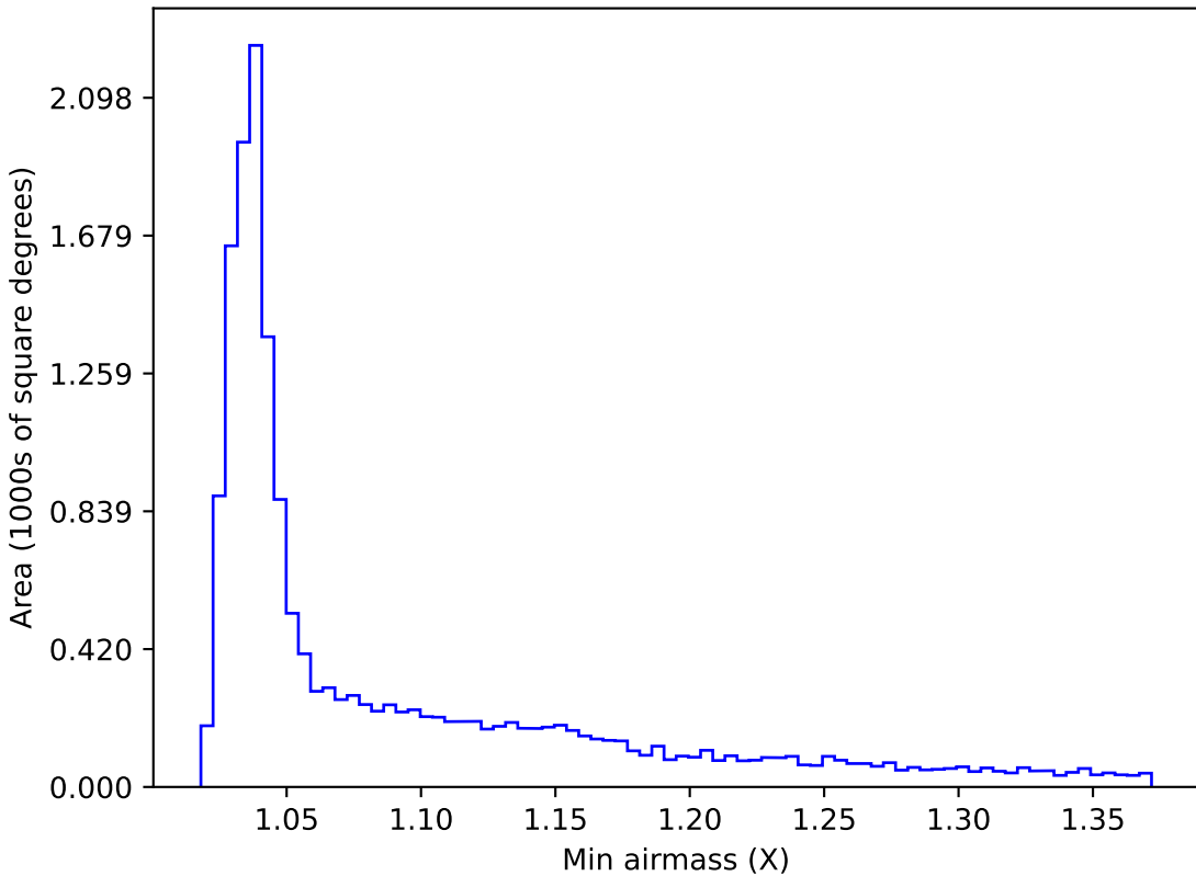
too_elab_r8_d3_griz_v3.4_10yrs WFD g band: Min airmass
