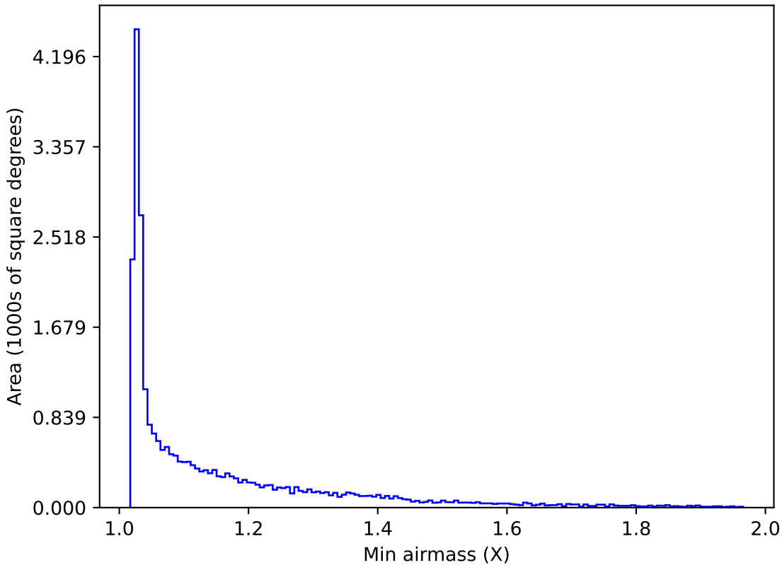
too_elab_r8_d3_griz_v3.4_10yrs All sky r band: Min airmass
