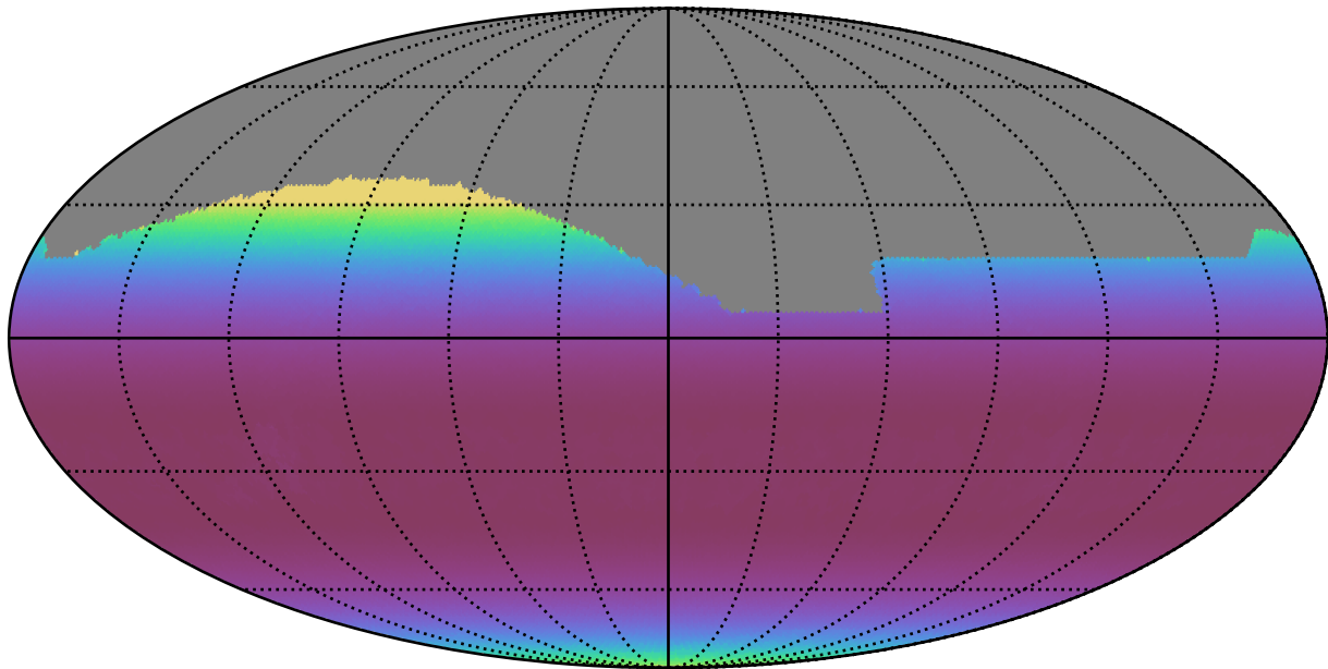
too_elab_r8_d3_griz_v3.4_10yrs All sky all bands: Min airmass
