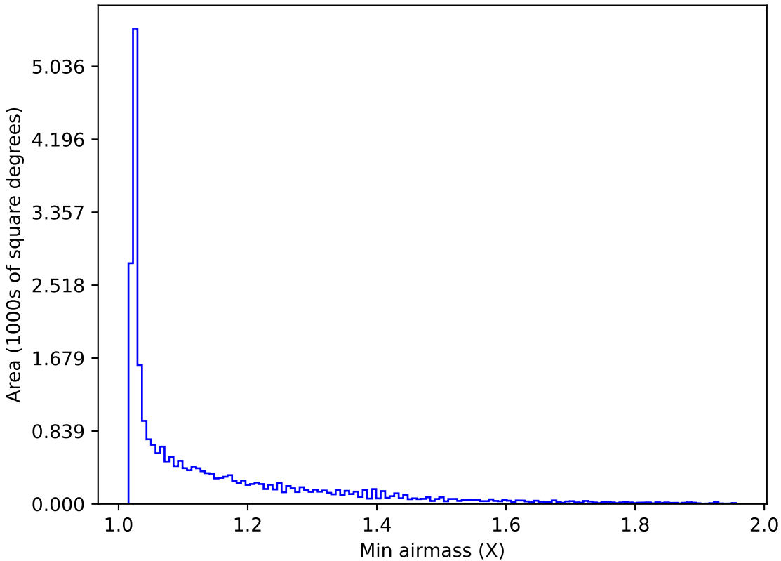
too_elab_r8_d3_griz_v3.4_10yrs All sky all bands: Min airmass
