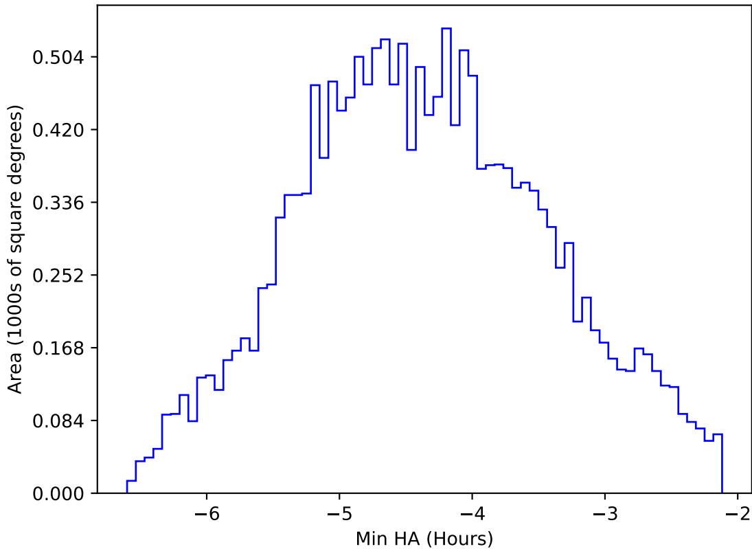
too_elab_r8_d3_griz_v3.4_10yrs WFD z band: Min HA
