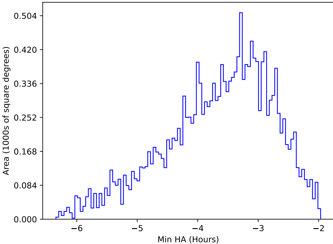
too_elab_r8_d3_griz_v3.4_10yrs WFD y band: Min HA
