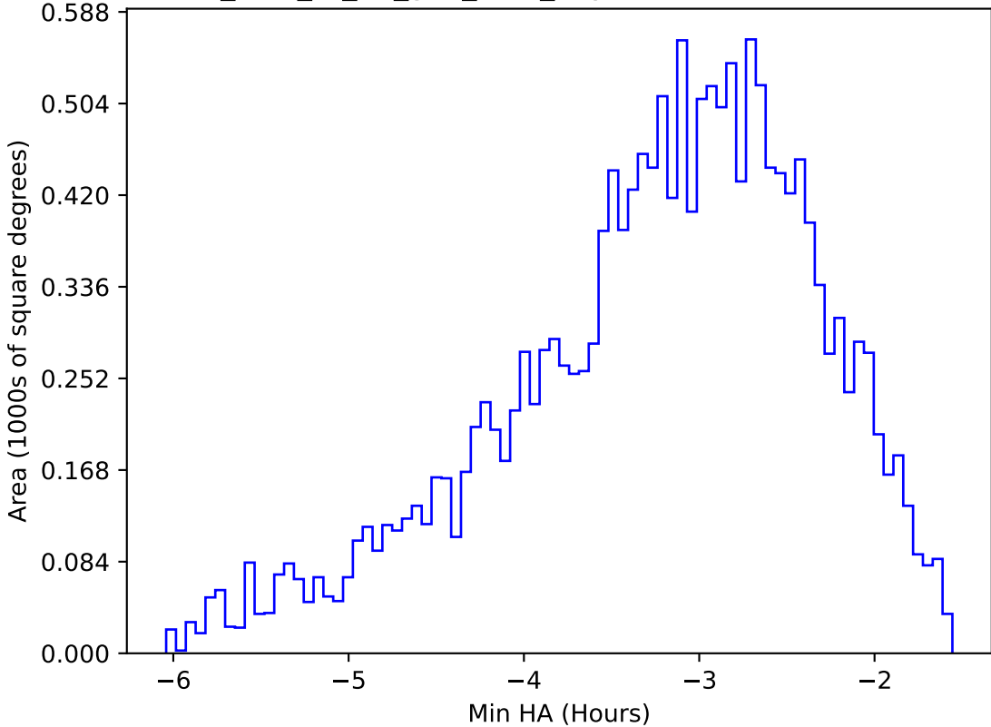
too_elab_r8_d3_griz_v3.4_10yrs WFD u band: Min HA
