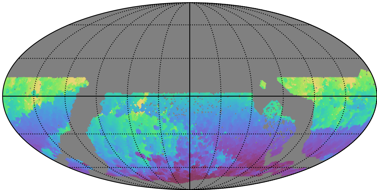
too_elab_r8_d3_griz_v3.4_10yrs WFD r band: Min HA
