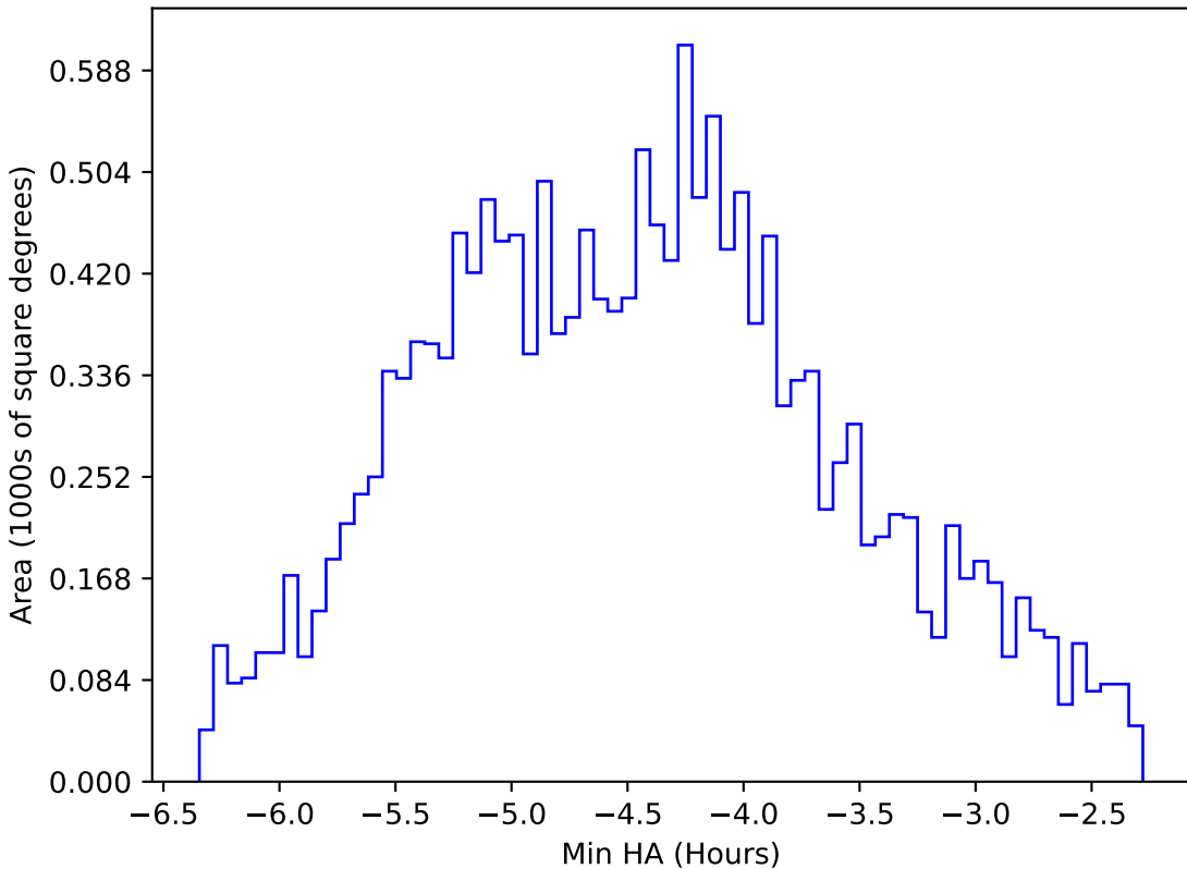
too_elab_r8_d3_griz_v3.4_10yrs WFD r band: Min HA
