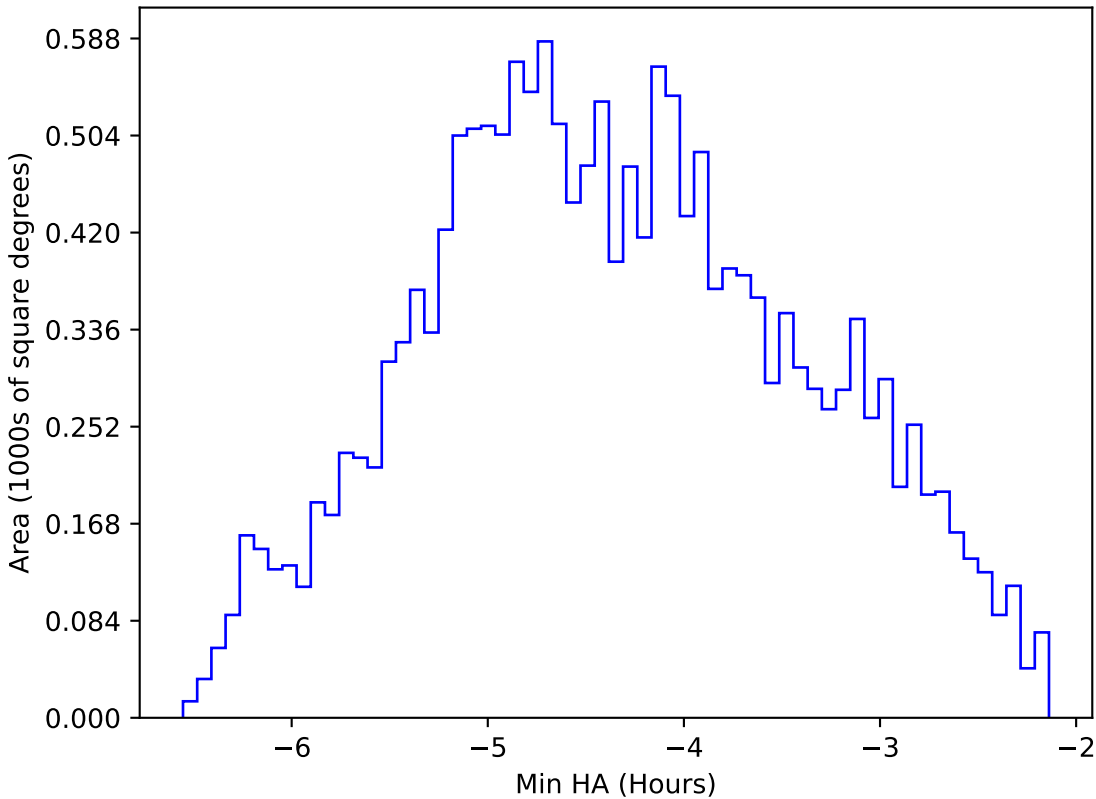
too_elab_r8_d3_griz_v3.4_10yrs WFD i band: Min HA
