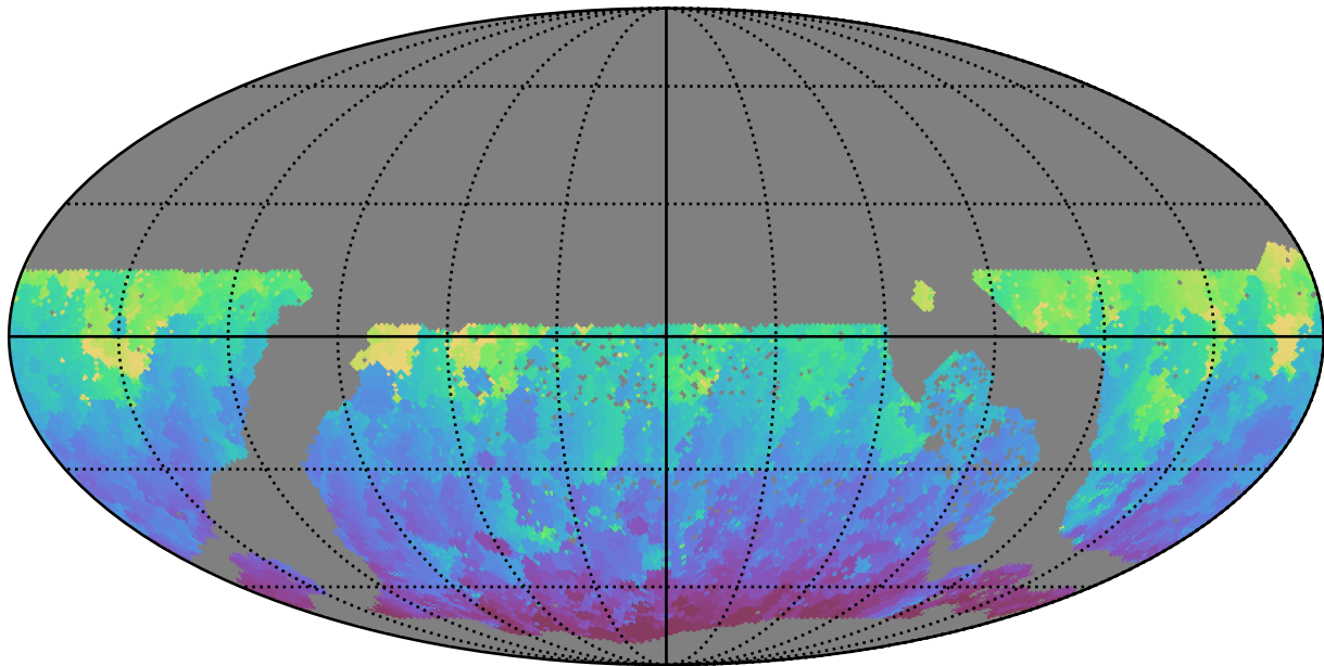
too_elab_r8_d3_griz_v3.4_10yrs WFD g band: Min HA
