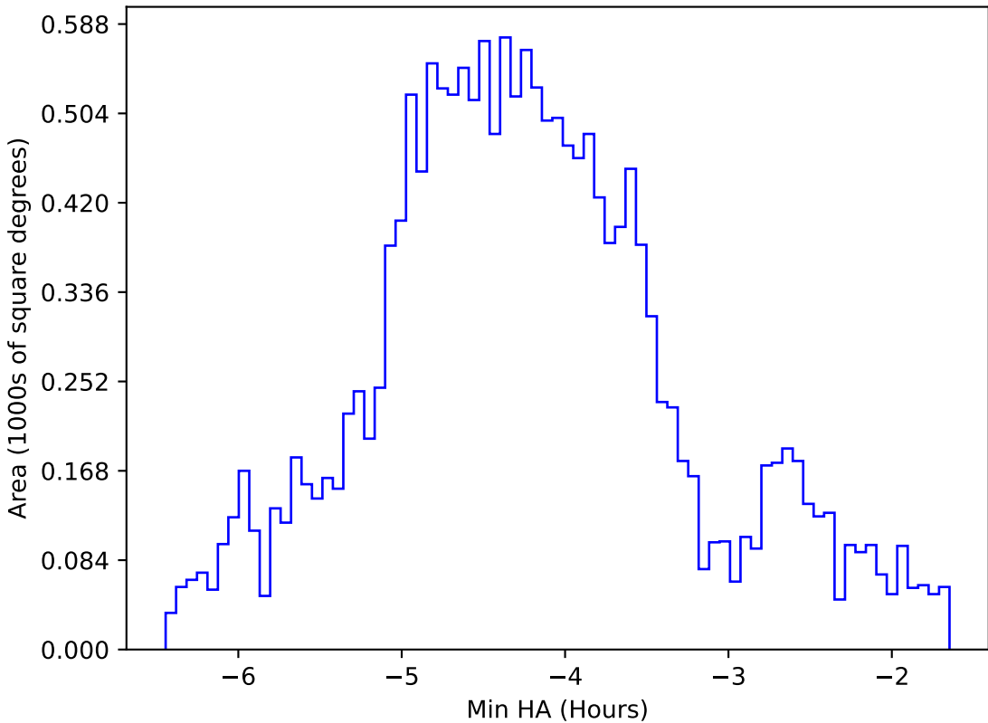
too_elab_r8_d3_griz_v3.4_10yrs WFD g band: Min HA
