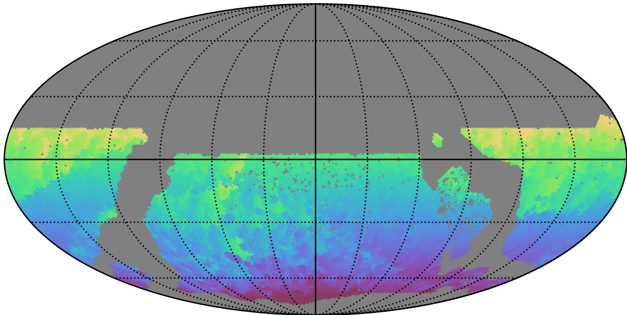
too_elab_r8_d3_griz_v3.4_10yrs WFD all bands: Min HA
