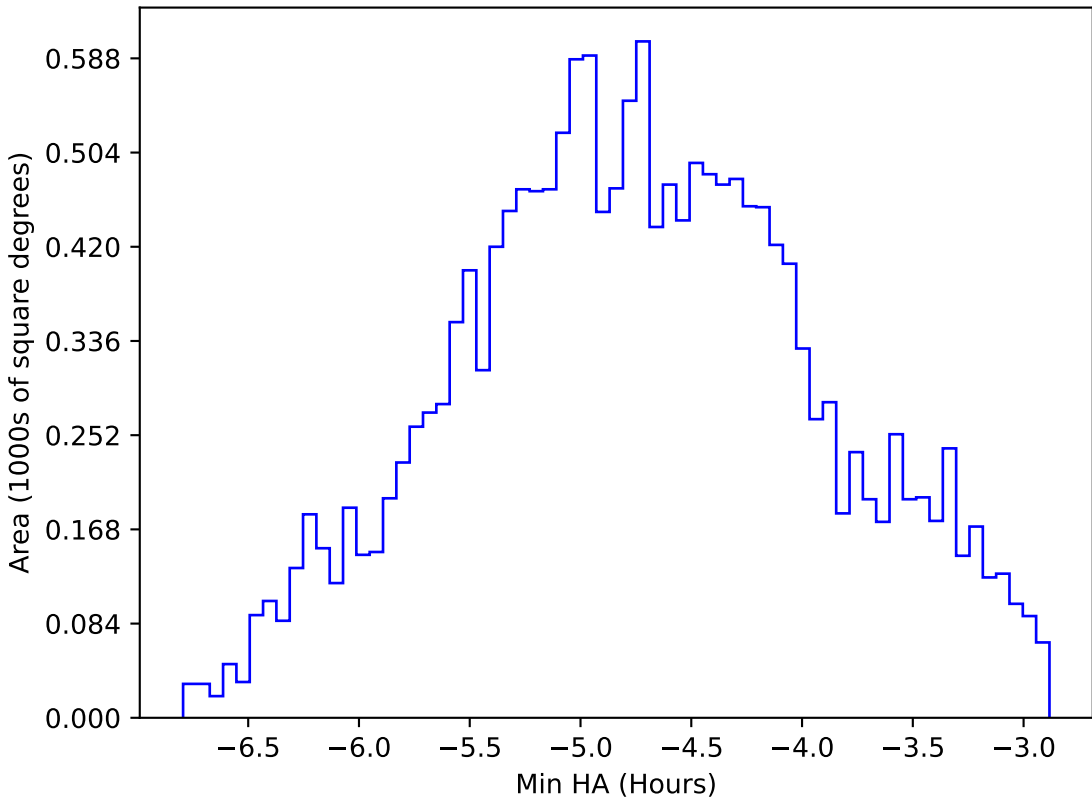
too_elab_r8_d3_griz_v3.4_10yrs WFD all bands: Min HA
