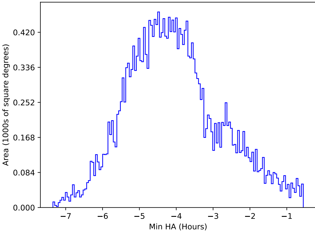
too_elab_r8_d3_griz_v3.4_10yrs All sky z band: Min HA
